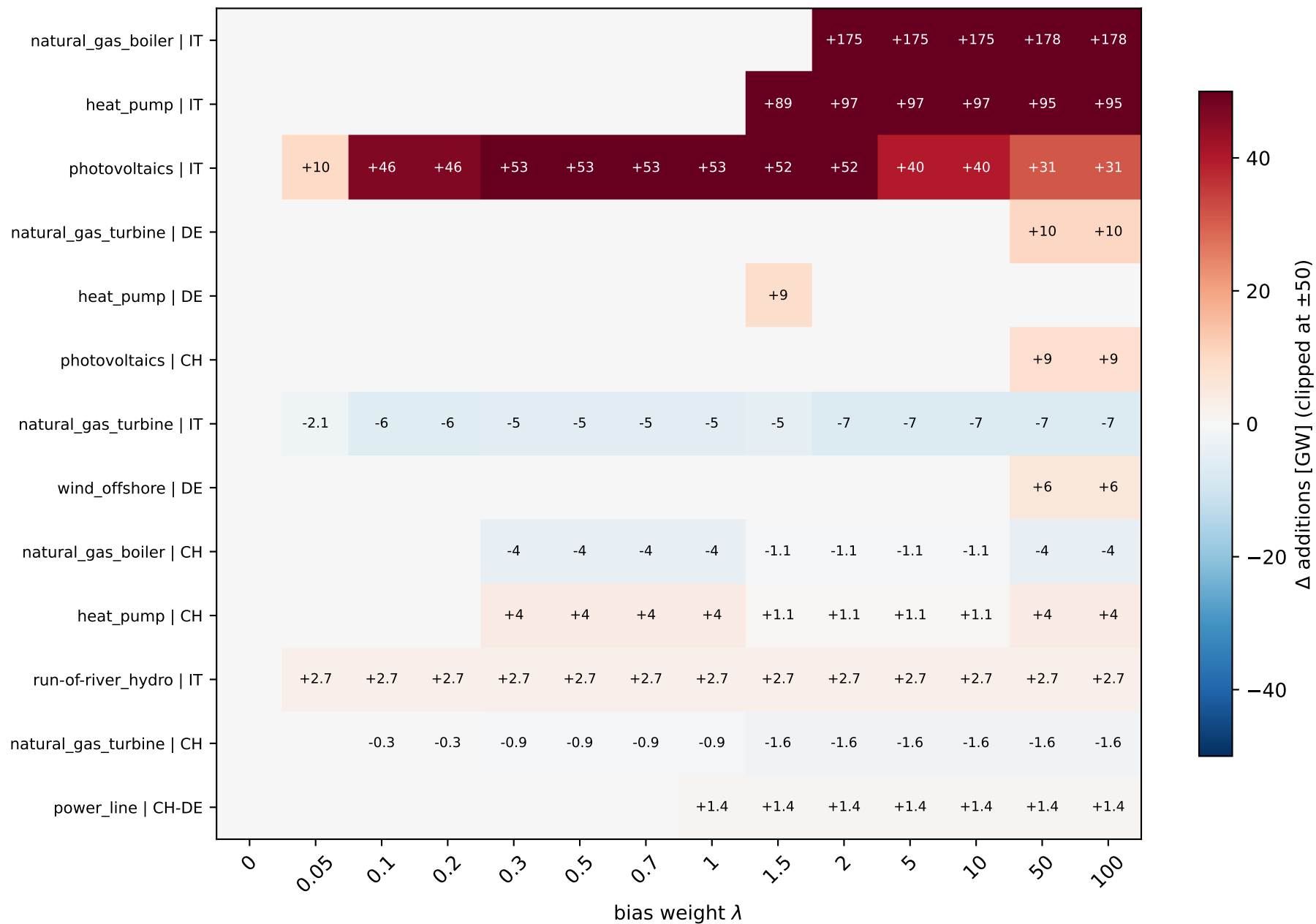
Change in total capacity additions vs. cost-optimal ( \lambda = 0 ) [GW]
